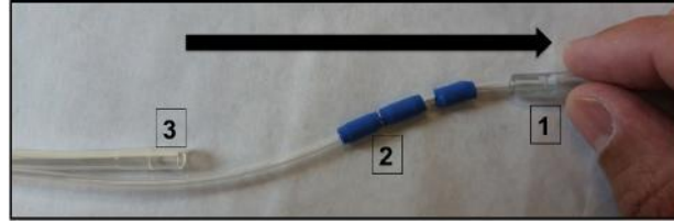
FIGURE 5: Hub (1) is passed retrograde through the peel away sheath first, followed by the blue compression guards (2) and then the end of the esophageal tube (3).
