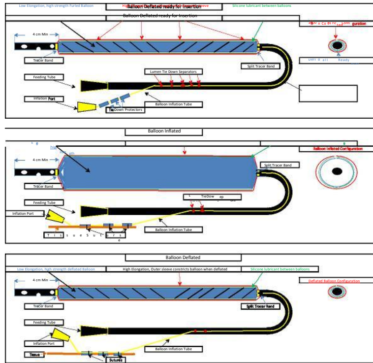
FIGURE 1: B-Tube double balloon design
